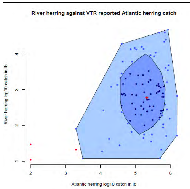
Figure A4. Bagplot of Log 10 observed River herring catch against log 10 VTR reported Atlantic herring catch. Red asterisk is location of bivariate median. Inner dark circle is middle 50% bivariate data with the greatest depth. The outer bag is 3X expansion of inner bag. Red points are considered “outside” values.
