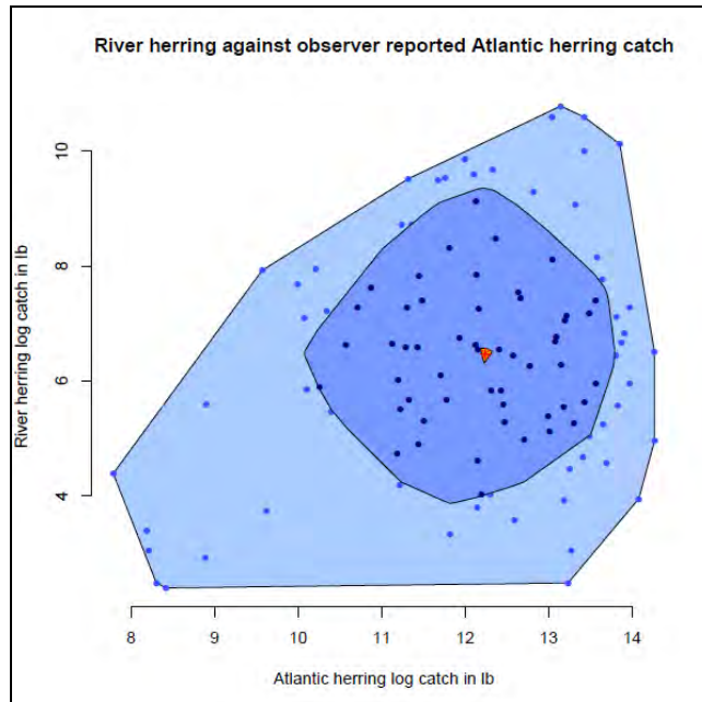
Figure A3. Bagplot of Log 10 observed River herring catch against log 10 Observer reported Atlantic herring catch. Red asterisk is location of bivariate median. Inner dark circle is middle 50% bivariate data with the greatest depth. The outer bag is 3X expansion of inner bag.
