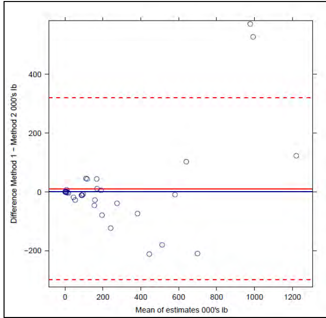
Figure C1: Comparison of river herring estimates using Method 1 and Method 2. Solid red line is mean difference (Method 1-Method 2). Dashed lines are mean difference \pm 2 standard deviations.
