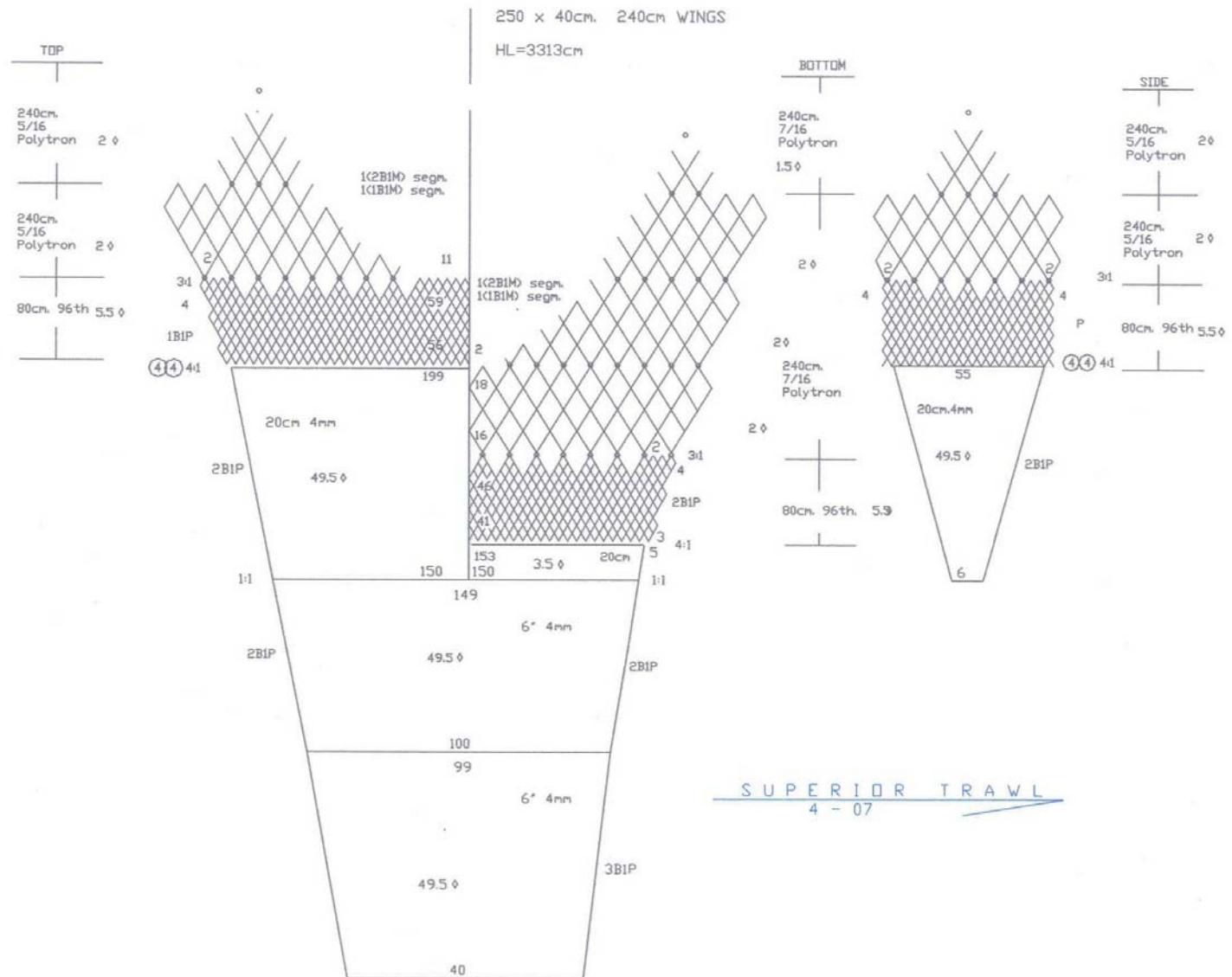
Figure 4. Net plan for the 250 x 40 cm Eliminator Trawl™.
