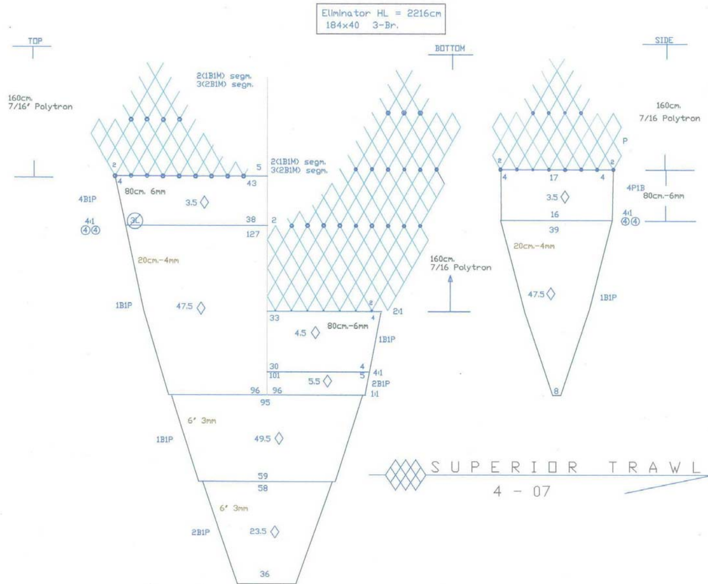
Figure 3. Net plan for the 184 x 40 cm Eliminator Trawl™.
