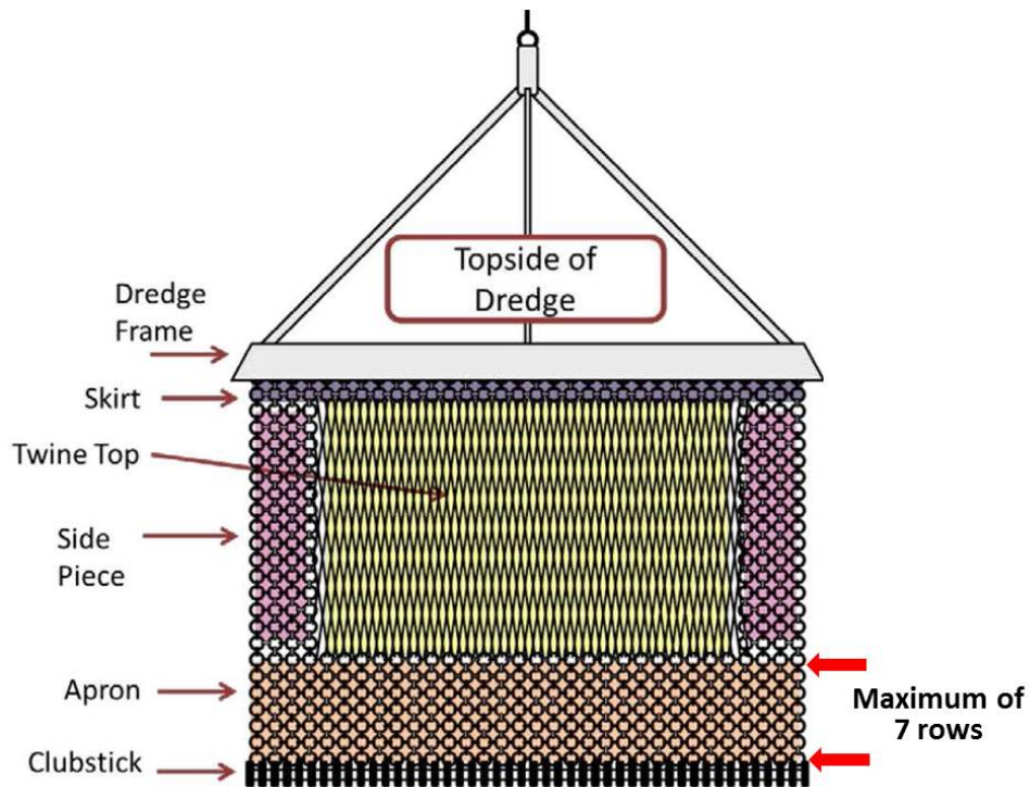
Dredge gear configuration required in the area west of 71° W. Long., excluding Mid-Atlantic access area
