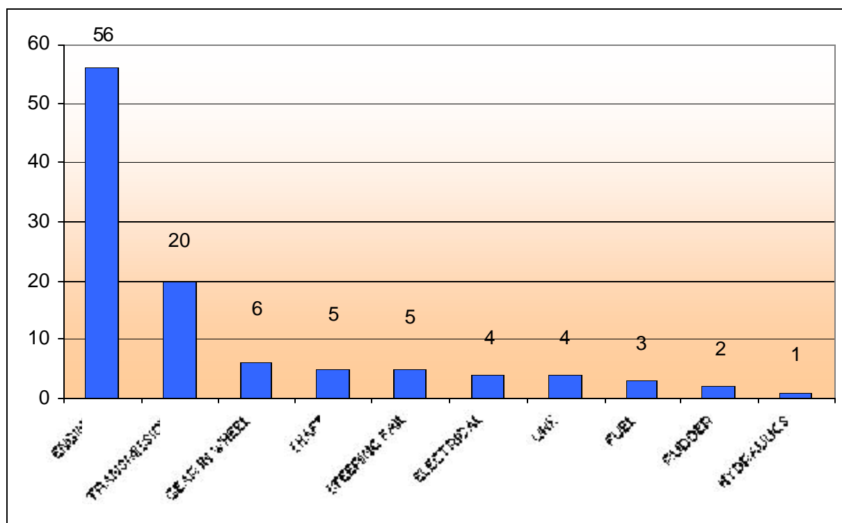
Figure 67. Most common causes of equipment casualties for offshore scallop vessels, 1993-2000.
