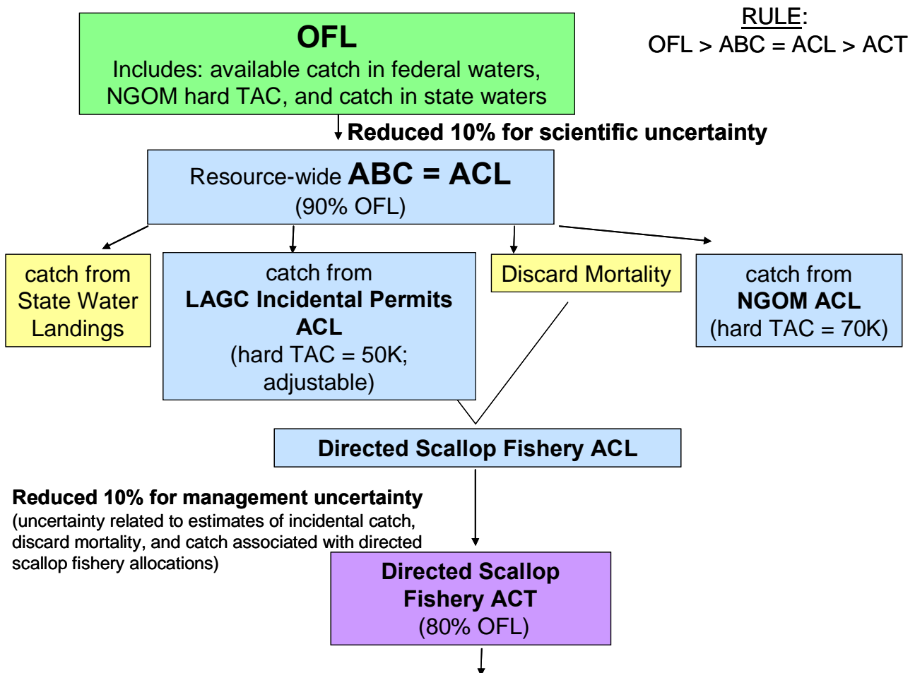
Figure 1. Schematic description of the revised general process for deriving OFL, ABC, ACL and ACT presented by the PDT.
