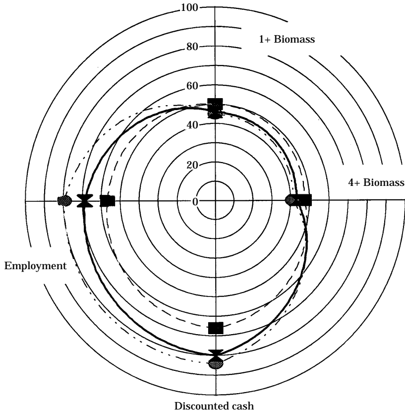
Figure 6. Radar graph of expected utilities from the four performance measures for the three strategies of —■— “decreasing”, - - - ⊙ - - - “constant”, and - · - · - · “increasing” TAC schedules of the case study.
